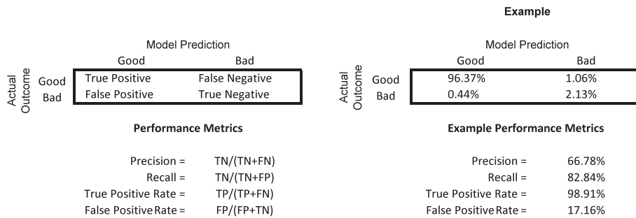
Fig. 14. Confusion matrix framework, model performance metrics, and numerical example based on December 2008 machine-learning forecasts of 90-days-or-more delinquencies over the 3-month forecast horizon from January to March 2009. Rows correspond to actual customer types (“Bad” is defined as 90-days-or more delinquent) and columns correspond to forecasted types. TN: True Negative, FN: False Negative, FP: False Positive; TP: True Positive.
