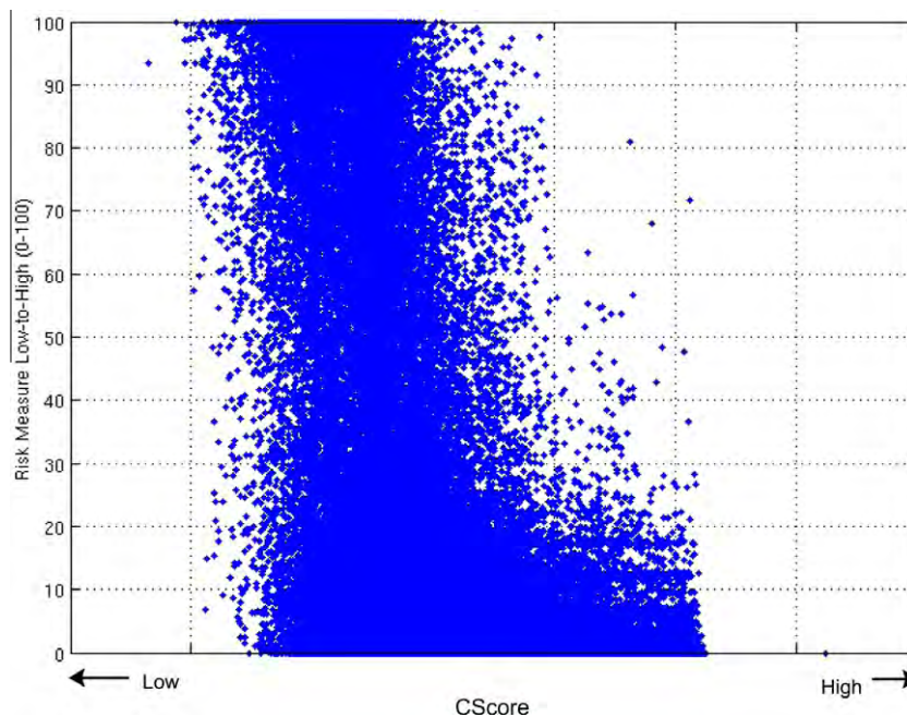
Fig. 12. Comparison of December 2008 CScore ( x -axis, and where higher values are associated with lower credit risk) and machine-learning forecasts of 90-days-or-more delinquency rates over subsequent 3-month windows using realized delinquency events from October to December 2008 and September 2008 feature vectors. Once calibrated, the machine-learning model is applied to the December 2008 feature vector, and the resulting "fitted values" are plotted ( y -axis) against the December 2008 CScores.
