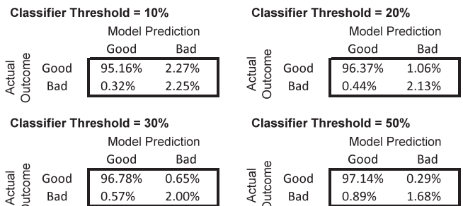
Fig. 15. Confusion matrices of machine-learning forecasts of 90-days-or-more delinquencies for four classification thresholds. Rows correspond to actual customer types (“Bad” is defined as 90-days-or more delinquent). The numerical example is based on the December 2008 model forecast for the 3-month forecast horizon from January to March 2009.
