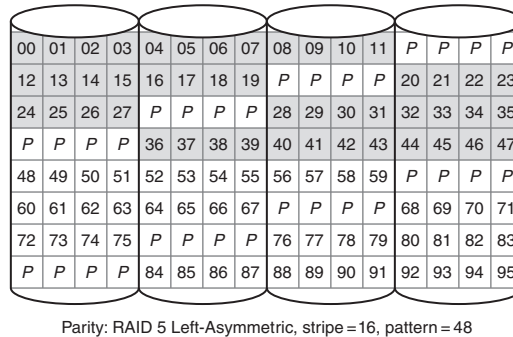
Figure D.29 A storage system with four disks, a chunk size of four 4 KB blocks, and using a RAID 5 Left-Asymmetric layout. Two repetitions of the pattern are shown.
